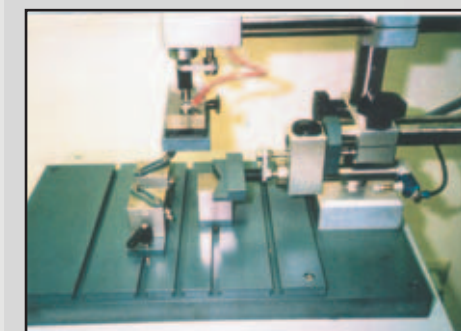
EMP 12 with pneumatic centering device for face-marking of round parts
