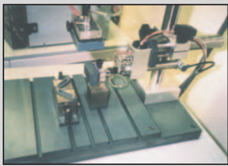
EMP 12 with a horizontal AND vertical marking unit for marking of round parts held in a prismatic jig
