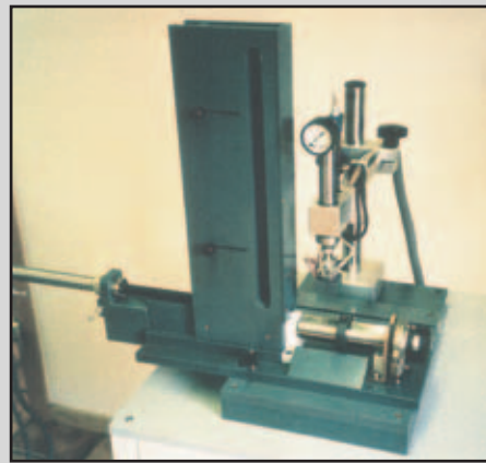
EMP 12 with magazine & feeding cylinder for marking cylindrical parts
