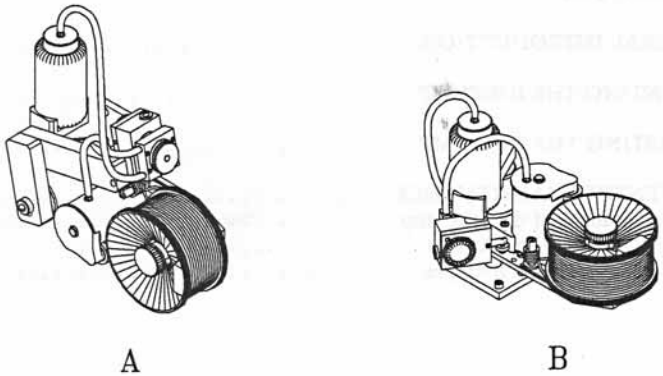
Figure 18 : Mounting possibilities for the inkpump
