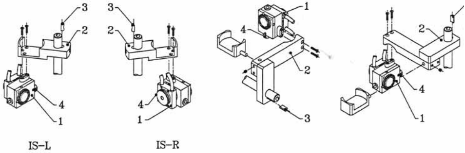
Figure 19 : Mounting the inkpump
