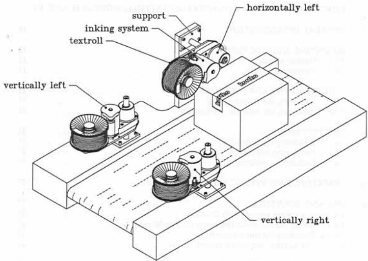
Figure 2 : Mounting possibilities
