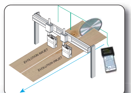
Printing description on timber exiting cutting system
